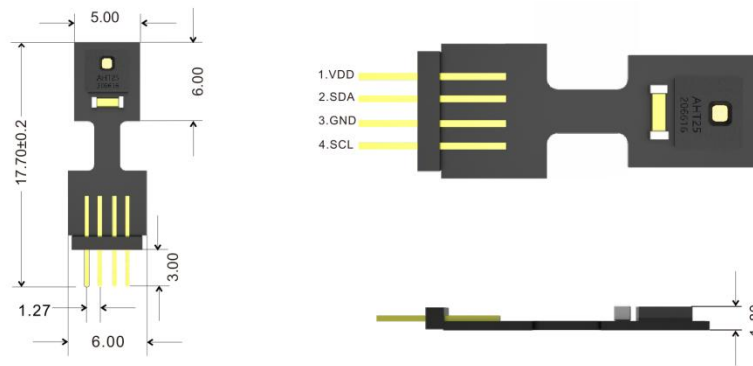
Figure 12. AHT25 sensor encapsulation (unit: mm unmarked tolerance: ± 0.1mm)
