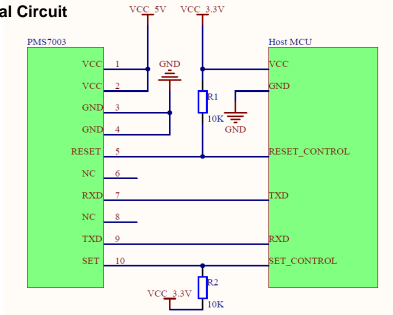
Figure 3 Typical Circuit
